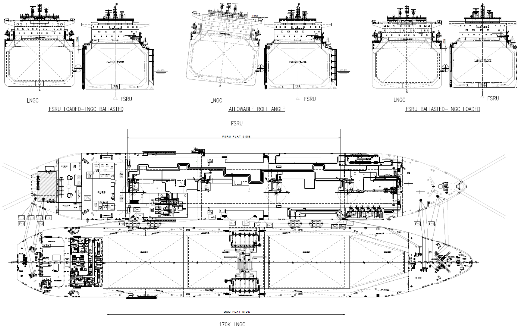
Figure 21 Proposed mooring plan with up to 170000 LNGC
