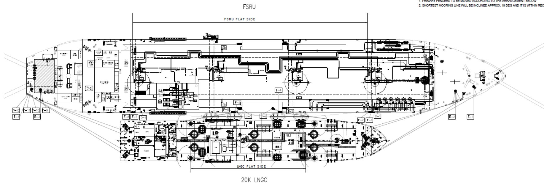
Figure 19 Proposed mooring plan with up to 20000 LNGC
