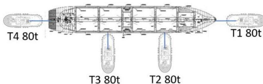
Figure 19 Typical Tug Arrangement
