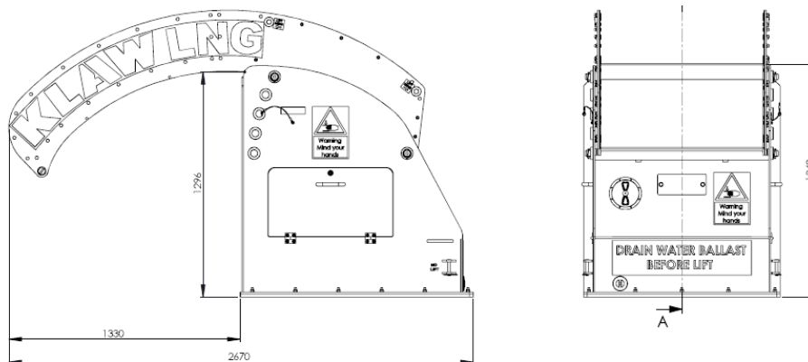
Figure 14 Saddles
