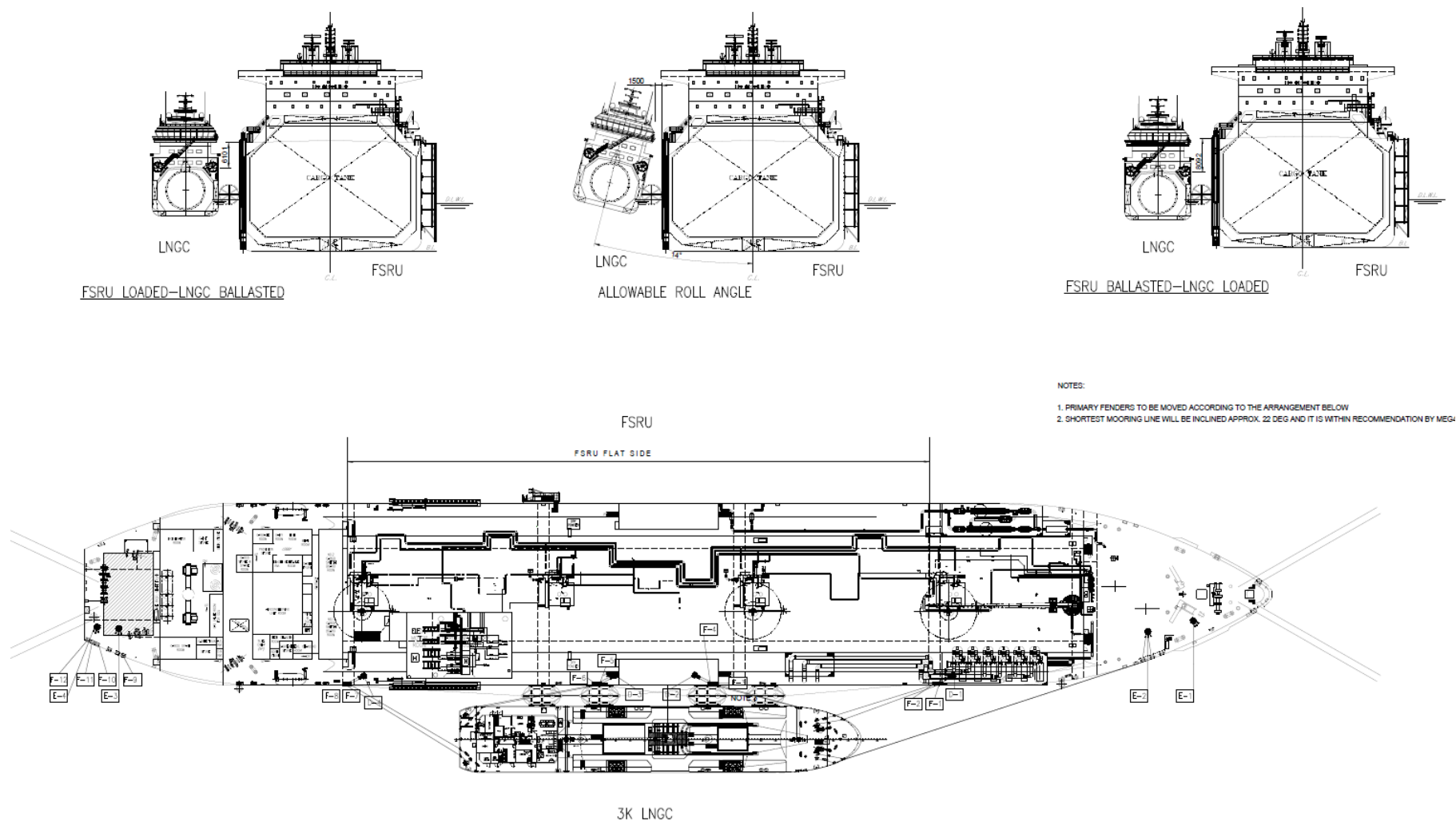
Figure 16 Proposed mooring plan with up to 3000 LNGC
