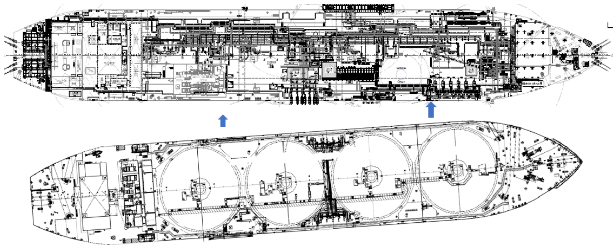
Figure 12 Angular Berthing
